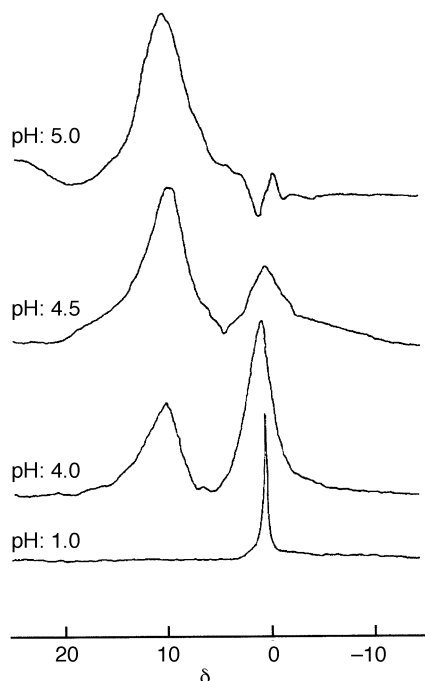
Fig. 8 Aluminium-27 NMR spectra of \text{Al}^{\text{III}} -Asp at 1:5 metal to amino acid ratio at different pH values; c_{\text{Al}} = 0.005 \text{ mol dm}^{-3}
